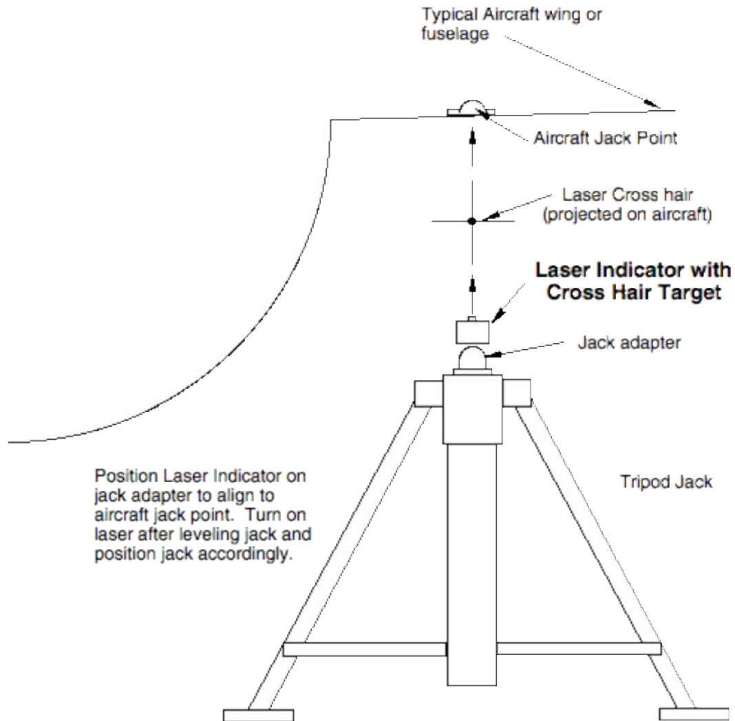
MALABAR Tripod Jack Laser Indicator
