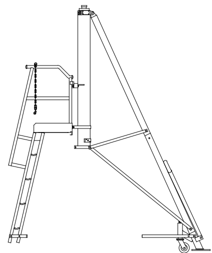
Model 713A shown with 48" Leg Extension Kit & Ladder/platform Kit (optional)
